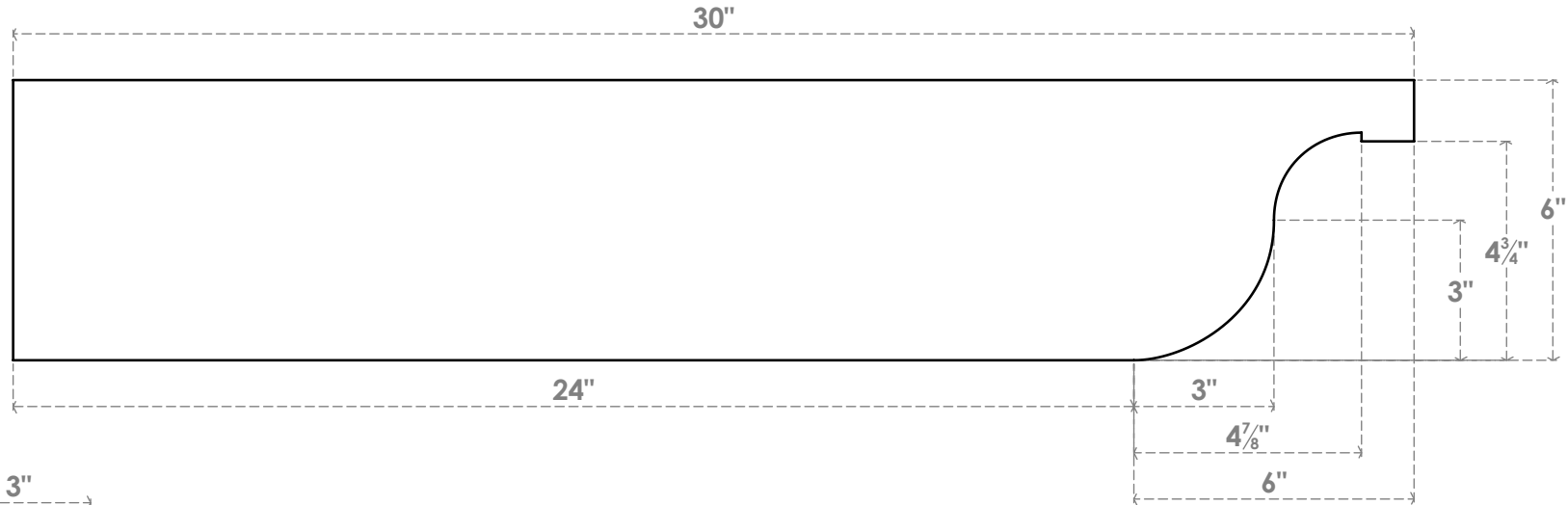
SIDE PROFILE
